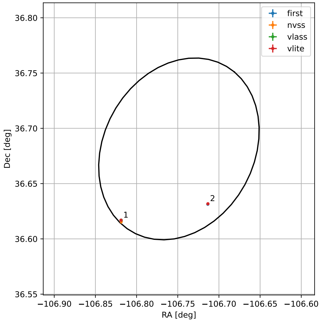
4FGL J1653.0+3640
