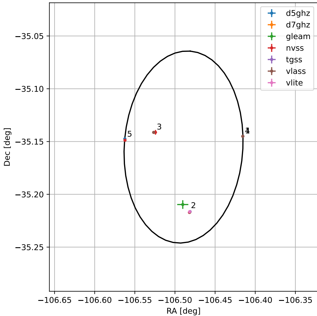
4FGL J1654.0-3509
