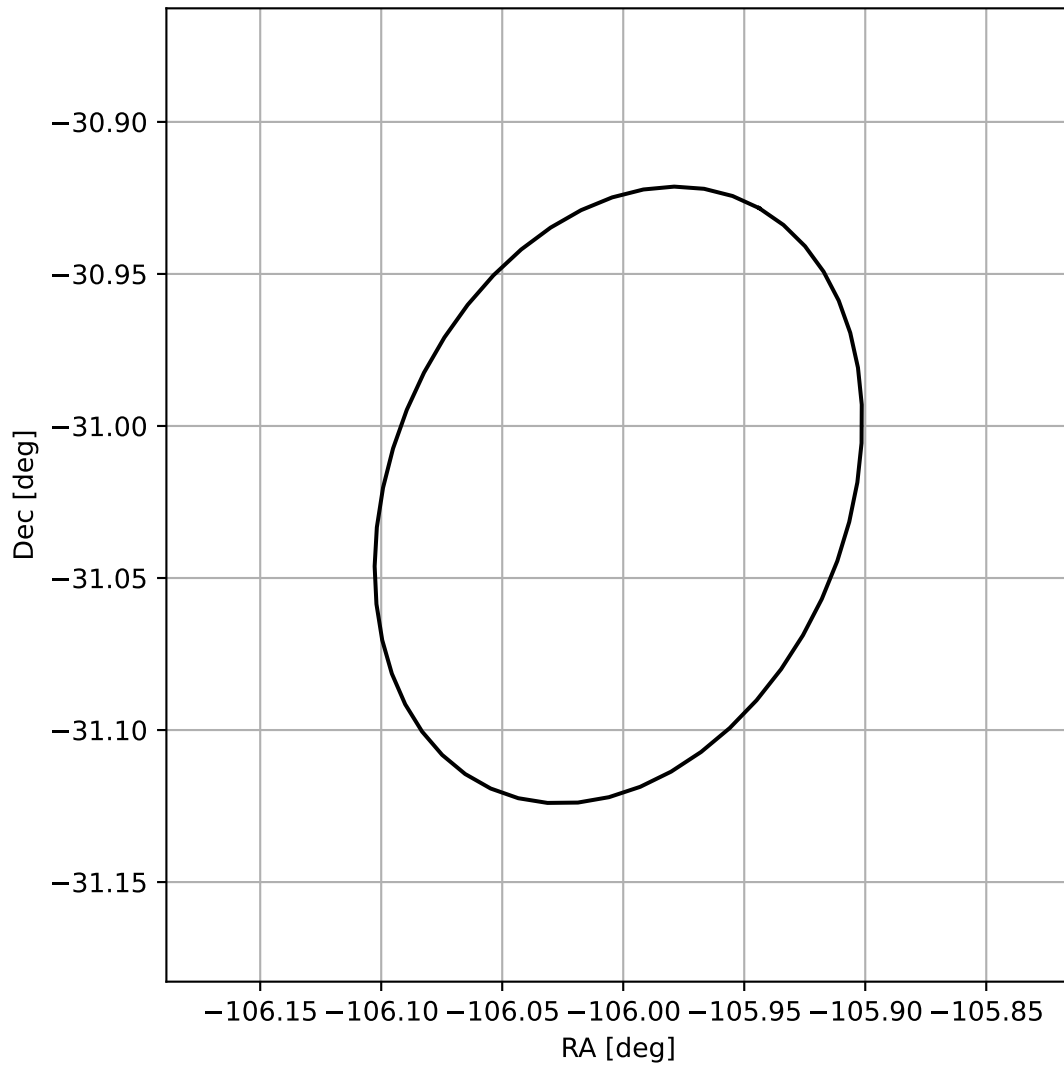
4FGL J1655.9-3101
