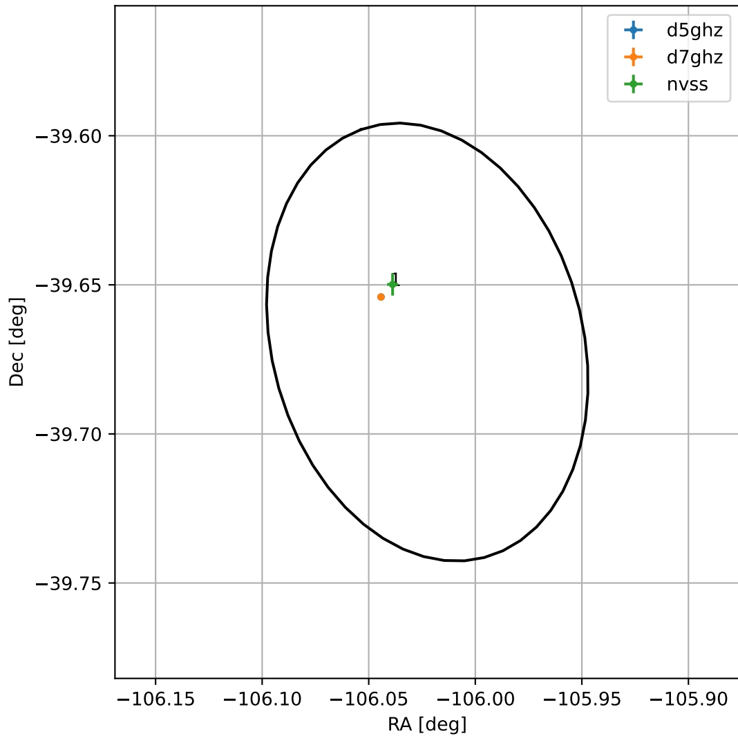
4FGL J1655.9-3940
