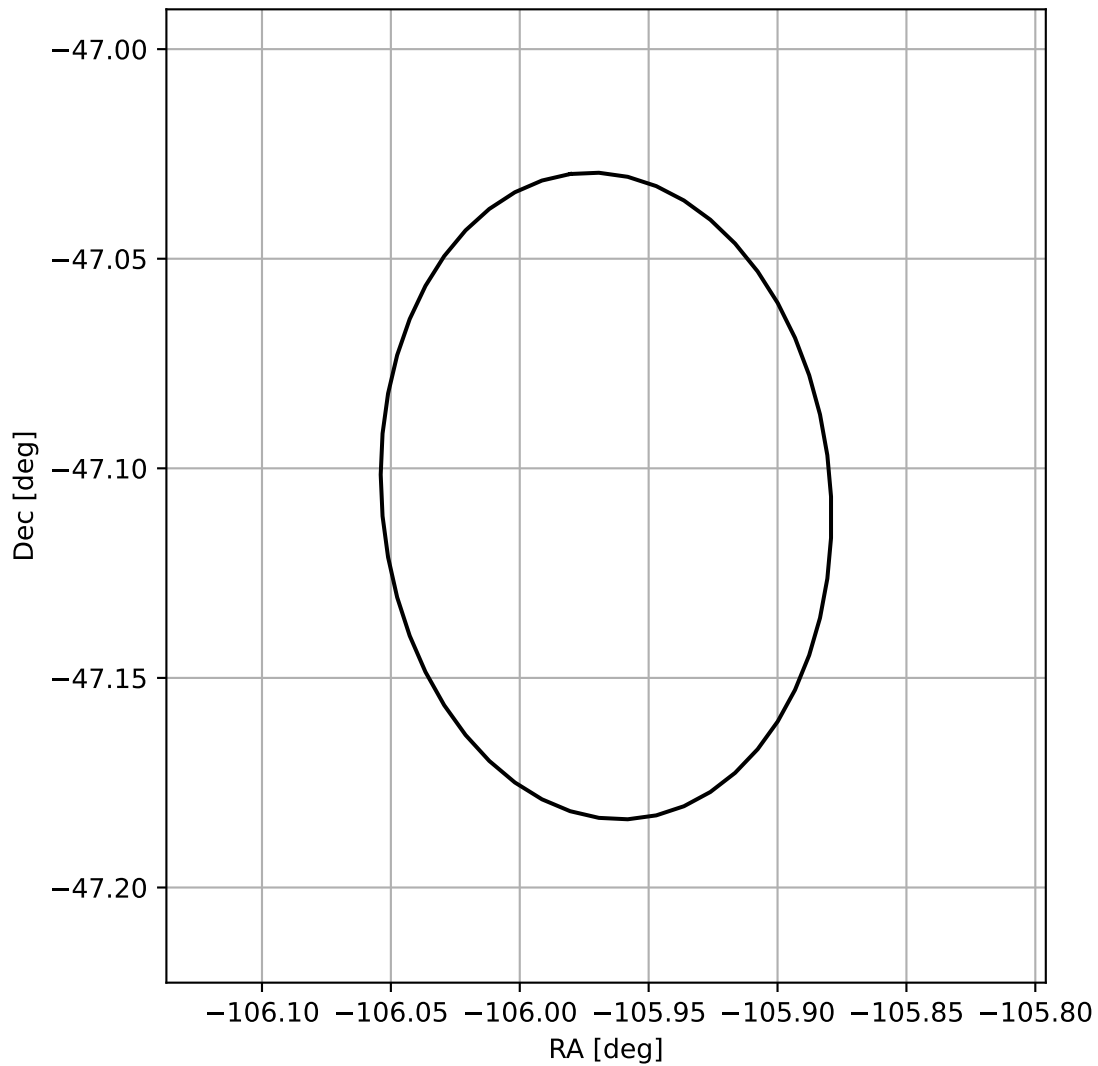
4FGL J1656.1-4706
