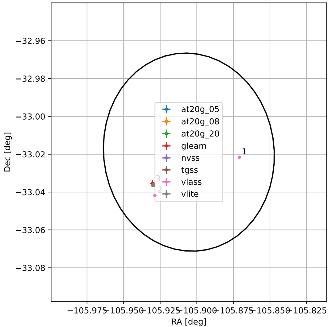
4FGL J1656.3-3301
