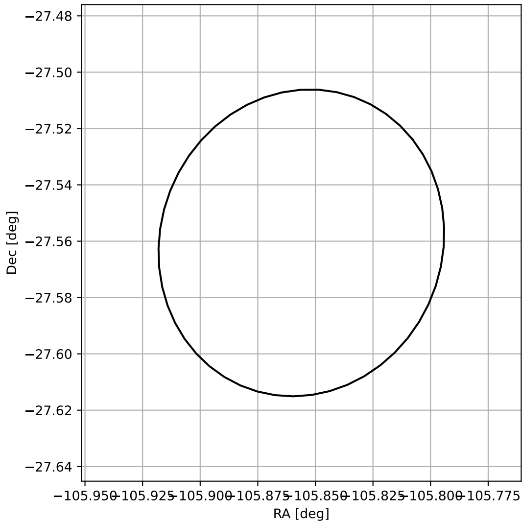
4FGL J1656.5-2733
