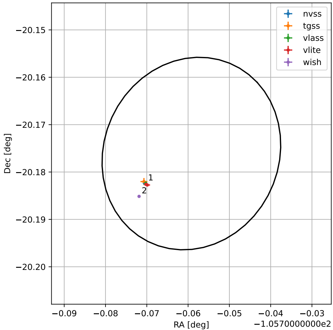
4FGL J1656.9-2010
