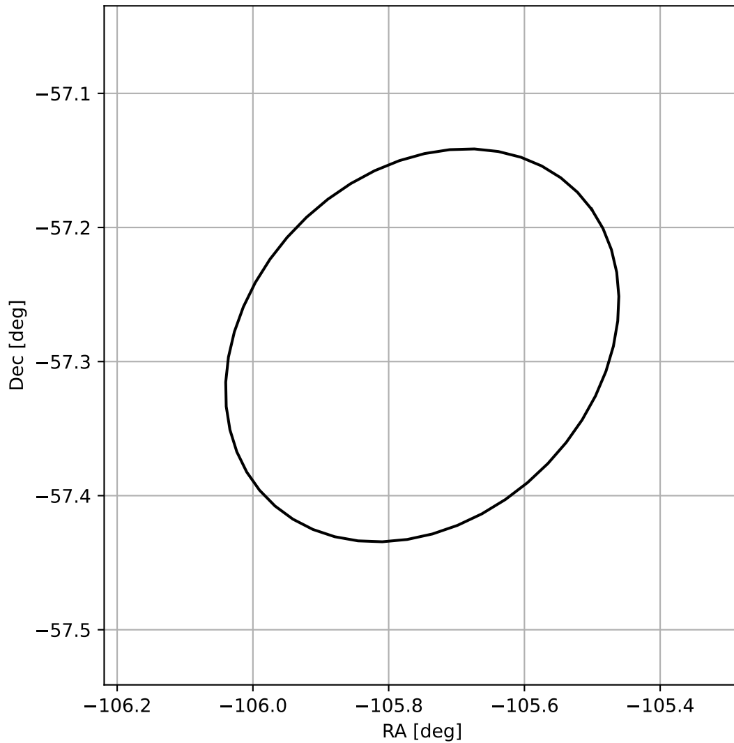
4FGL J1656.9-5717
