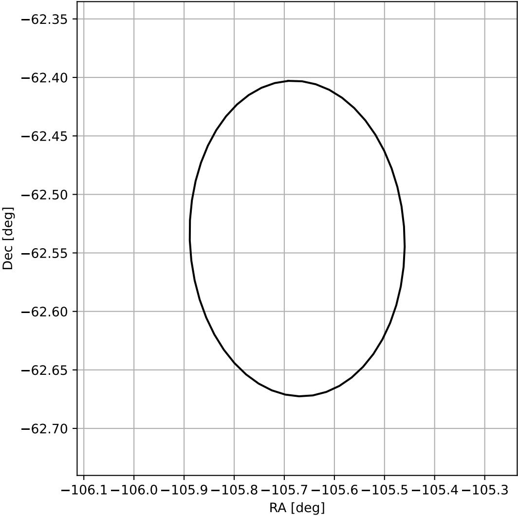
4FGL J1657.3-6232
