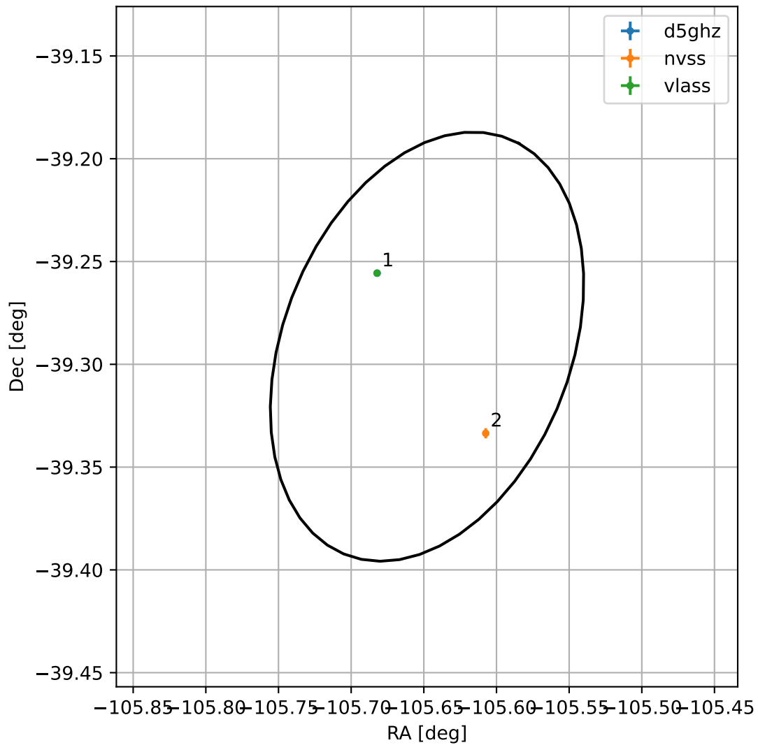
4FGL J1657.4-3917
