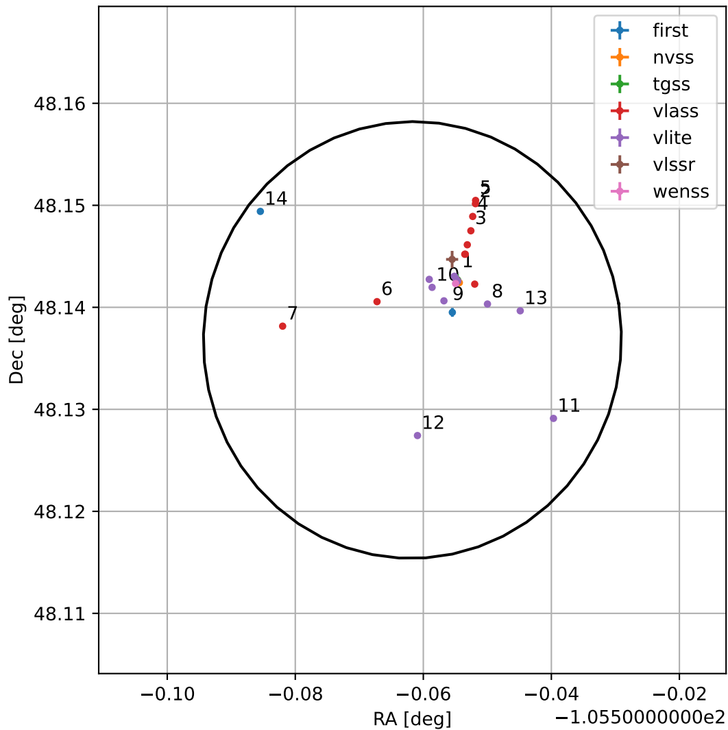
4FGL J1657.7+4808
