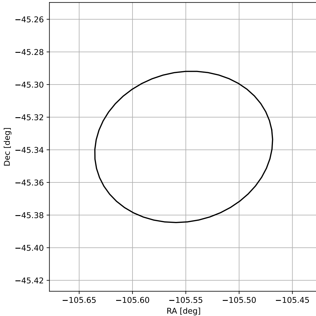
4FGL J1657.7-4520
