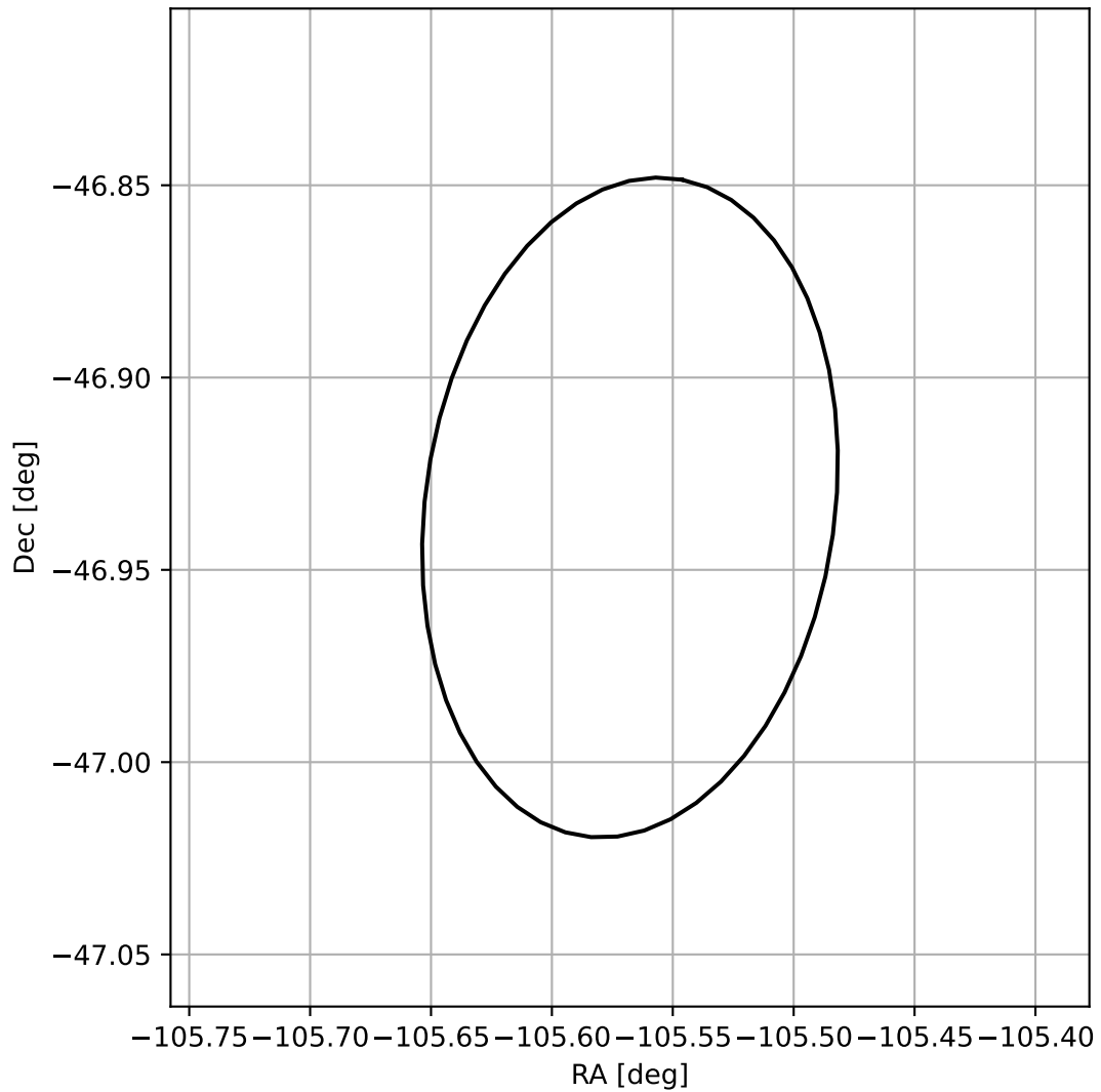
4FGL J1657.7-4656
