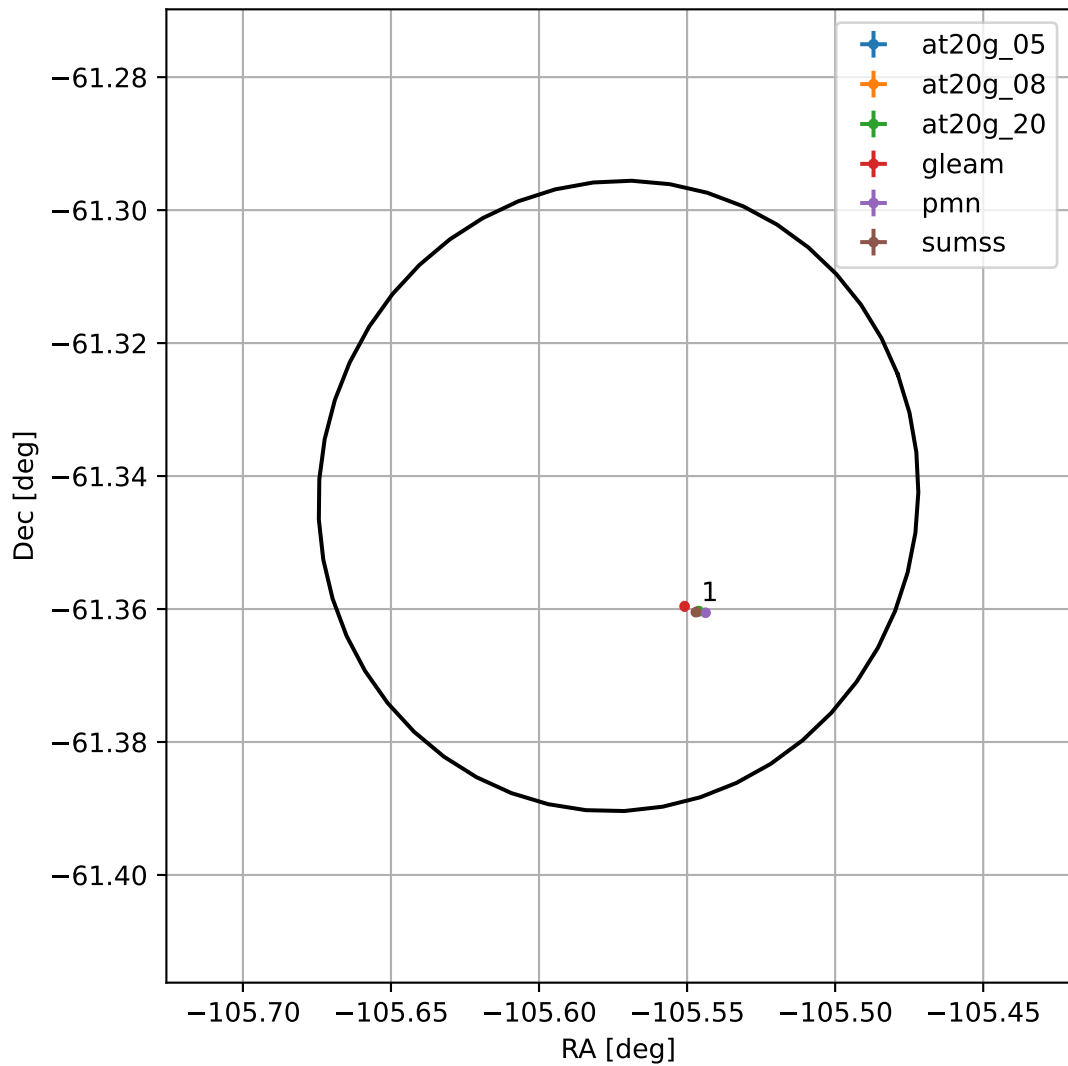
4FGL J1657.7-6120
