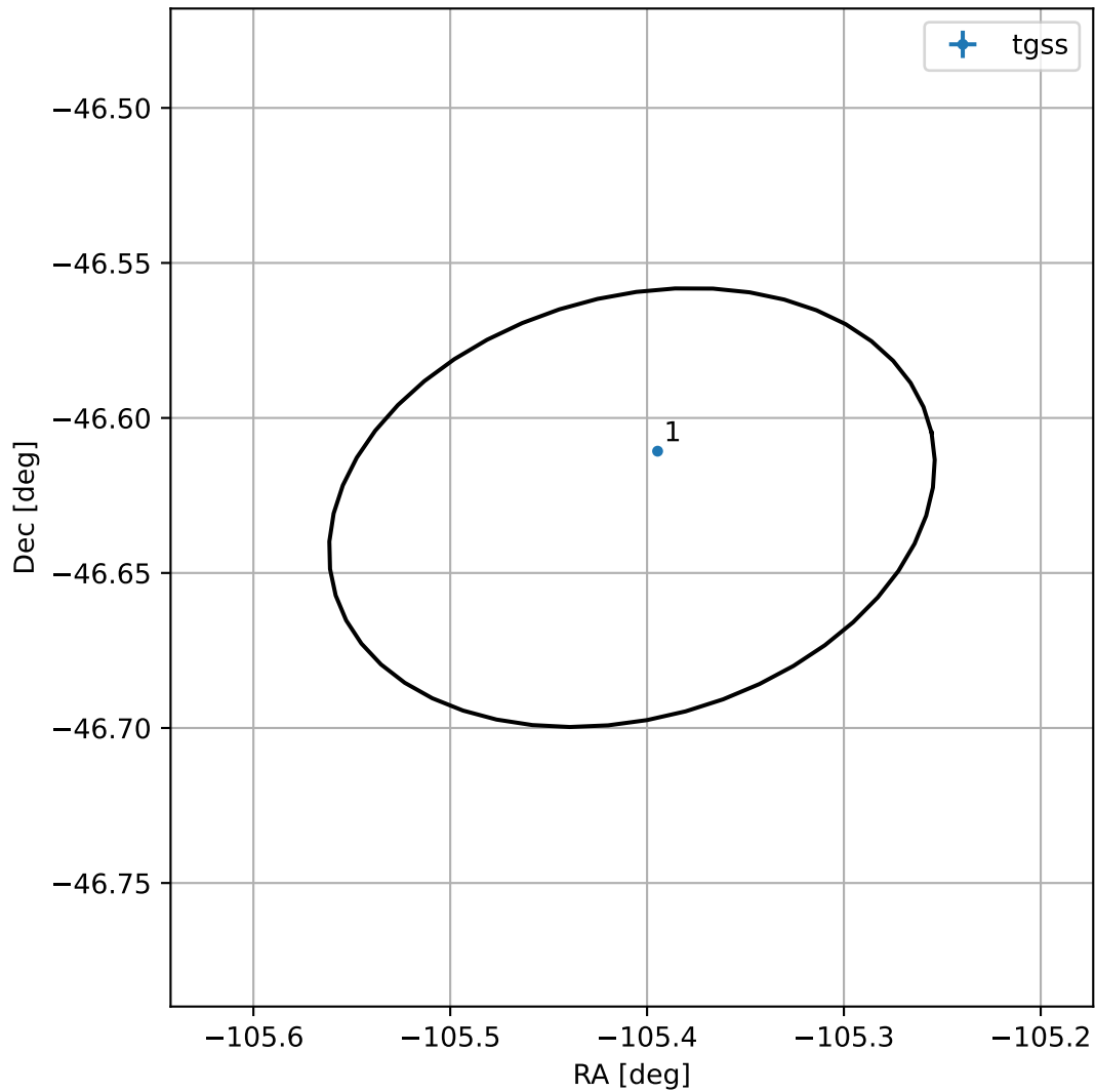
4FGL J1658.3-4637
