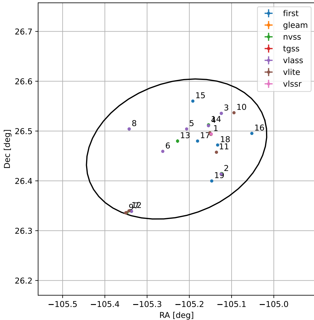
4FGL J1659.0+2627
