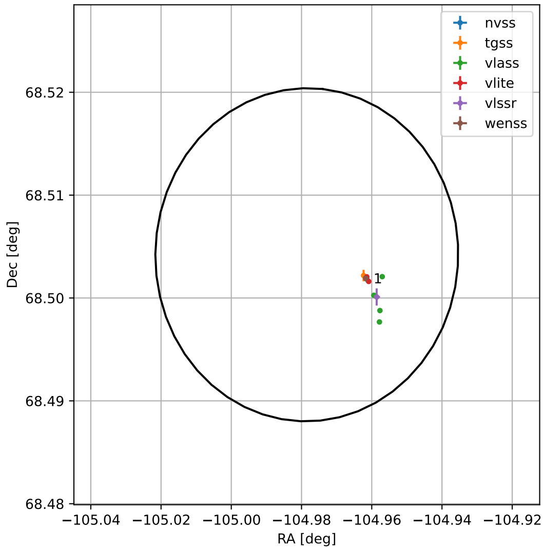
4FGL J1700.0+6830
