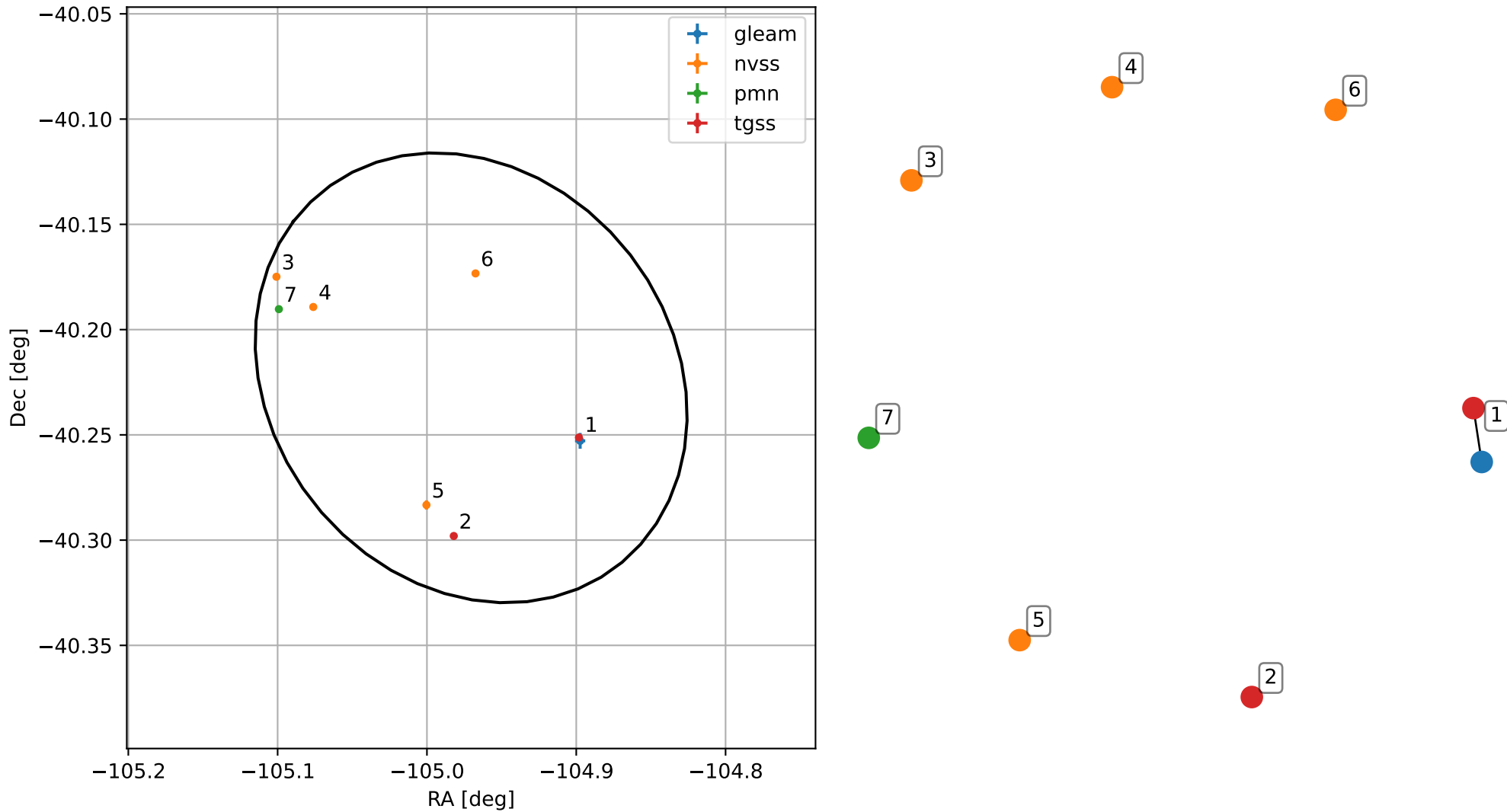
4FGL J1700.1-4013
