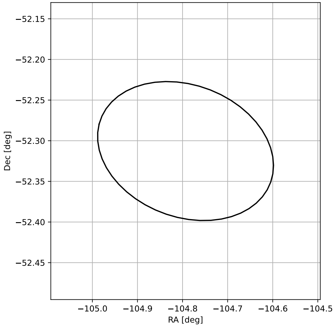
4FGL J1700.8-5218
