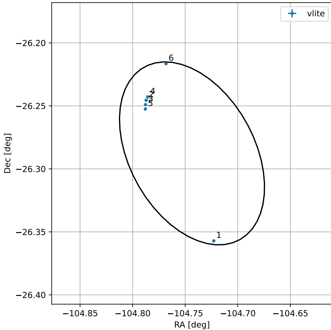
4FGL J1701.0-2617
