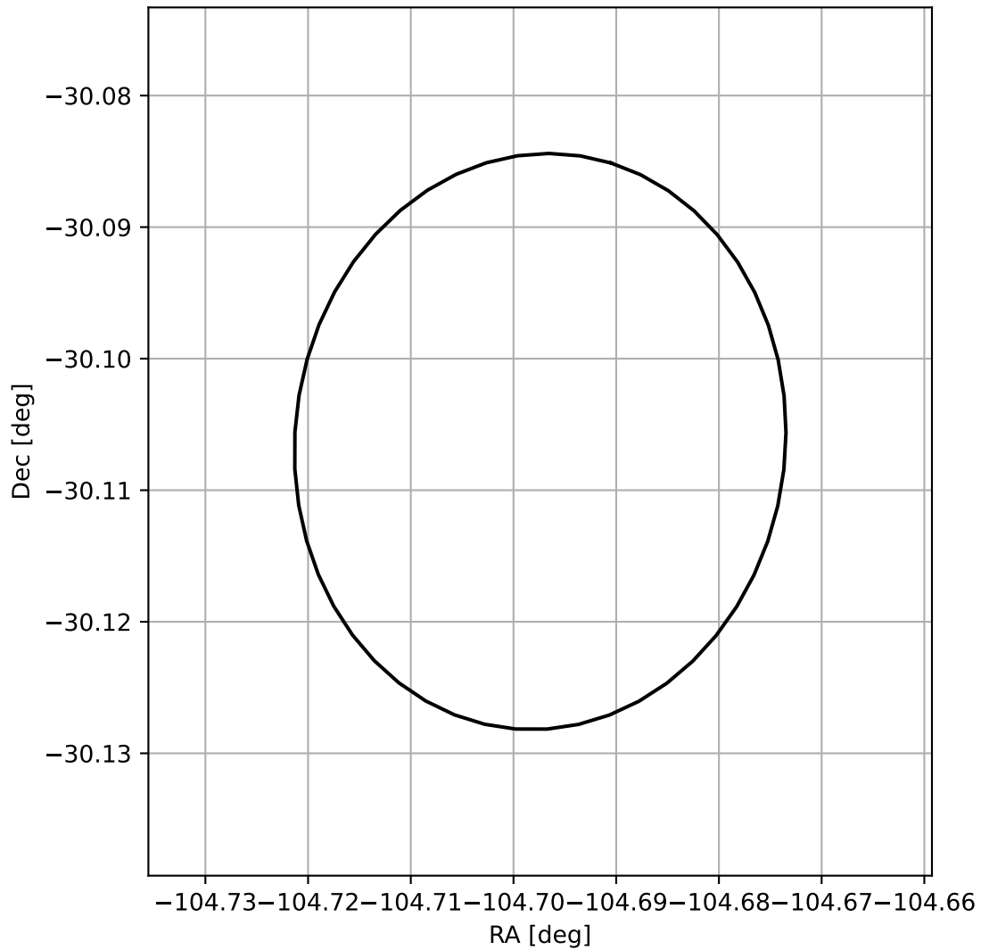
4FGL J1701.2-3006
