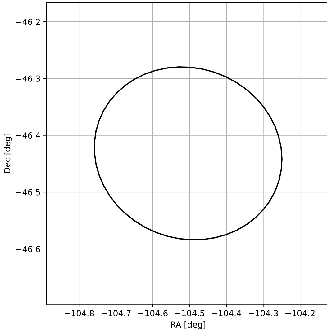
4FGL J1701.9-4625
