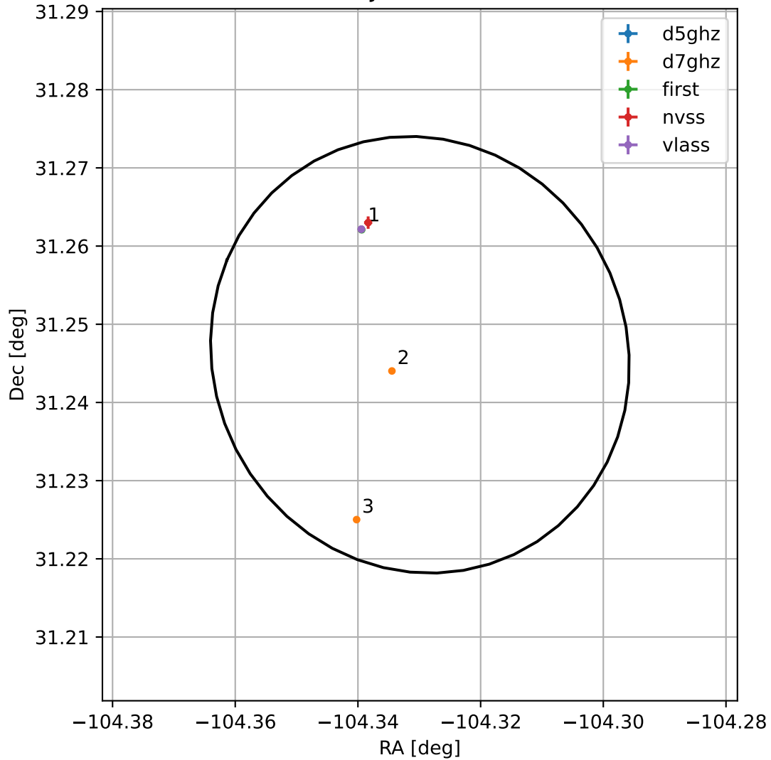
4FGL J1702.6+3114
