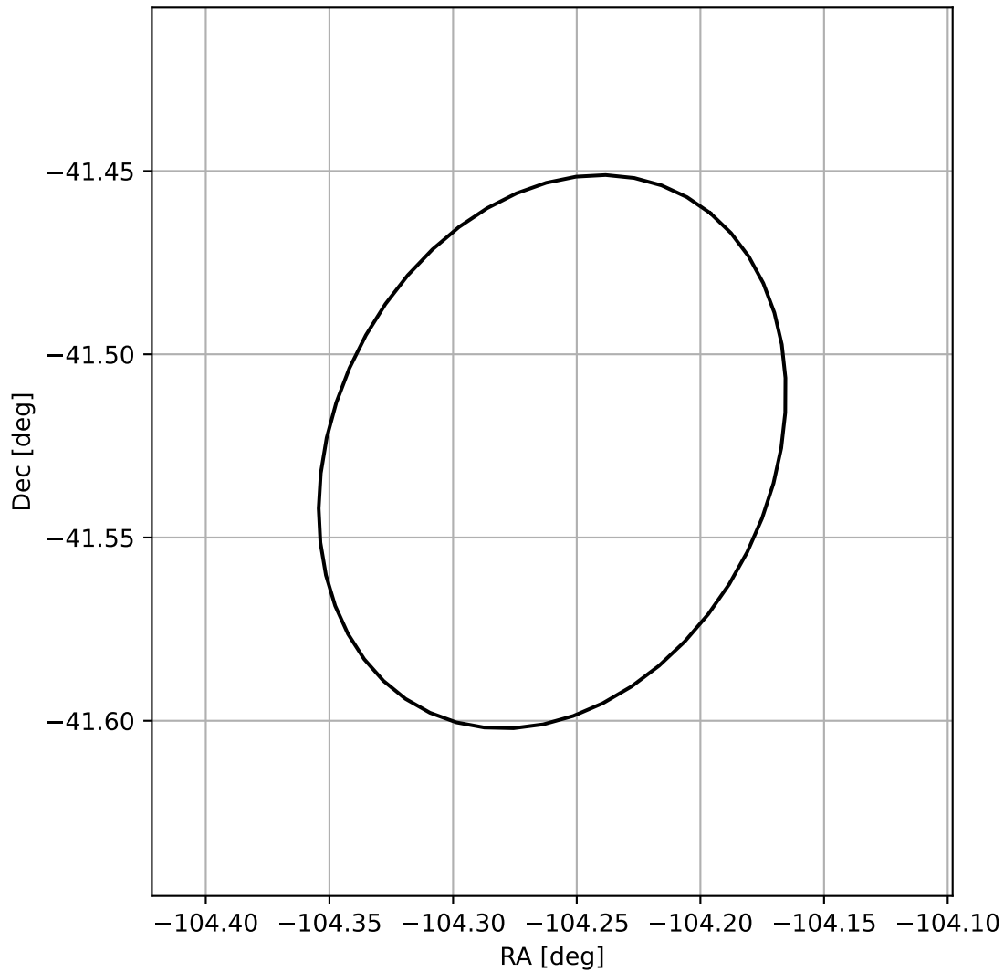
4FGL J1702.9-4131
