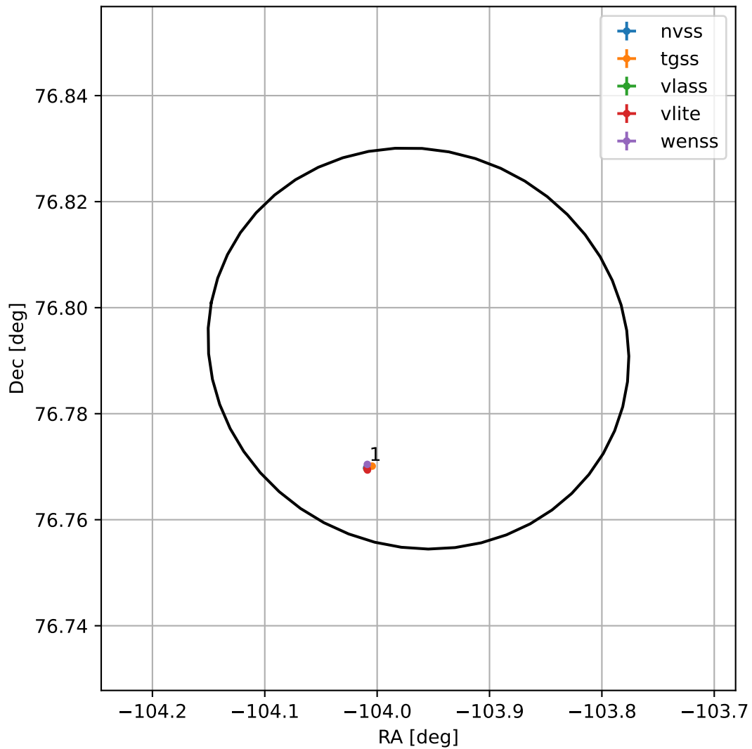
4FGL J1704.1+7647
