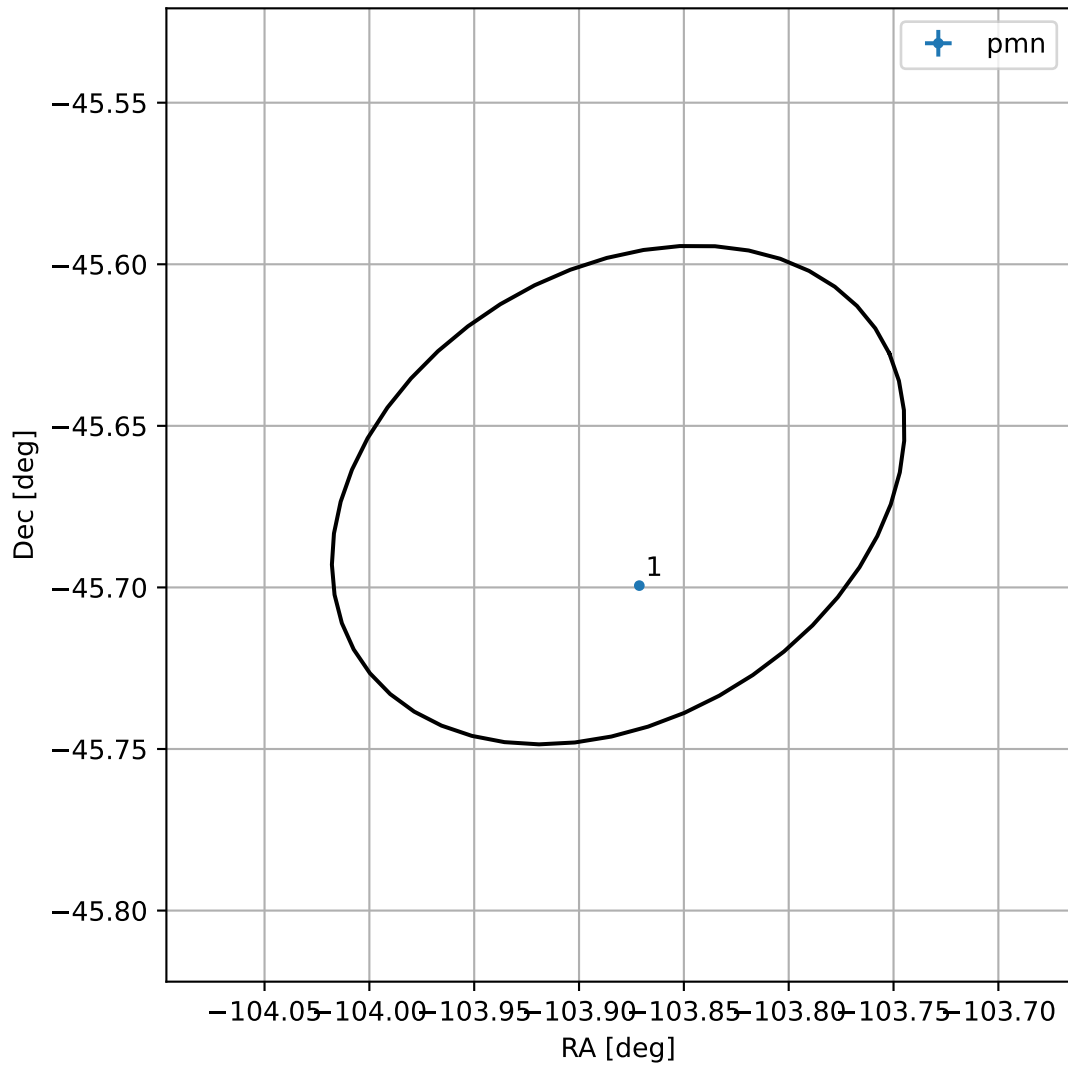
4FGL J1704.4-4540
