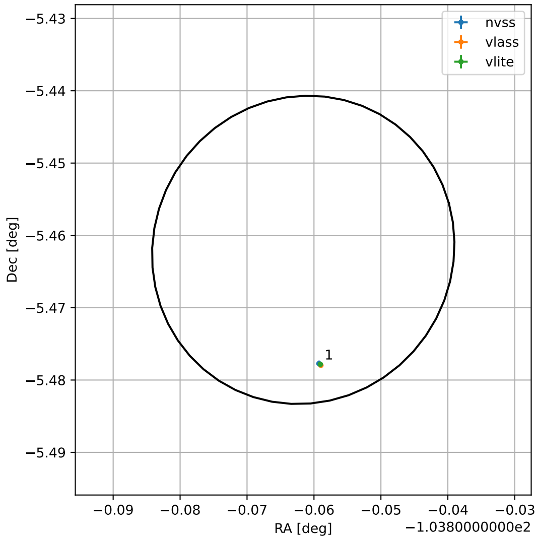
4FGL J1704.5-0527
