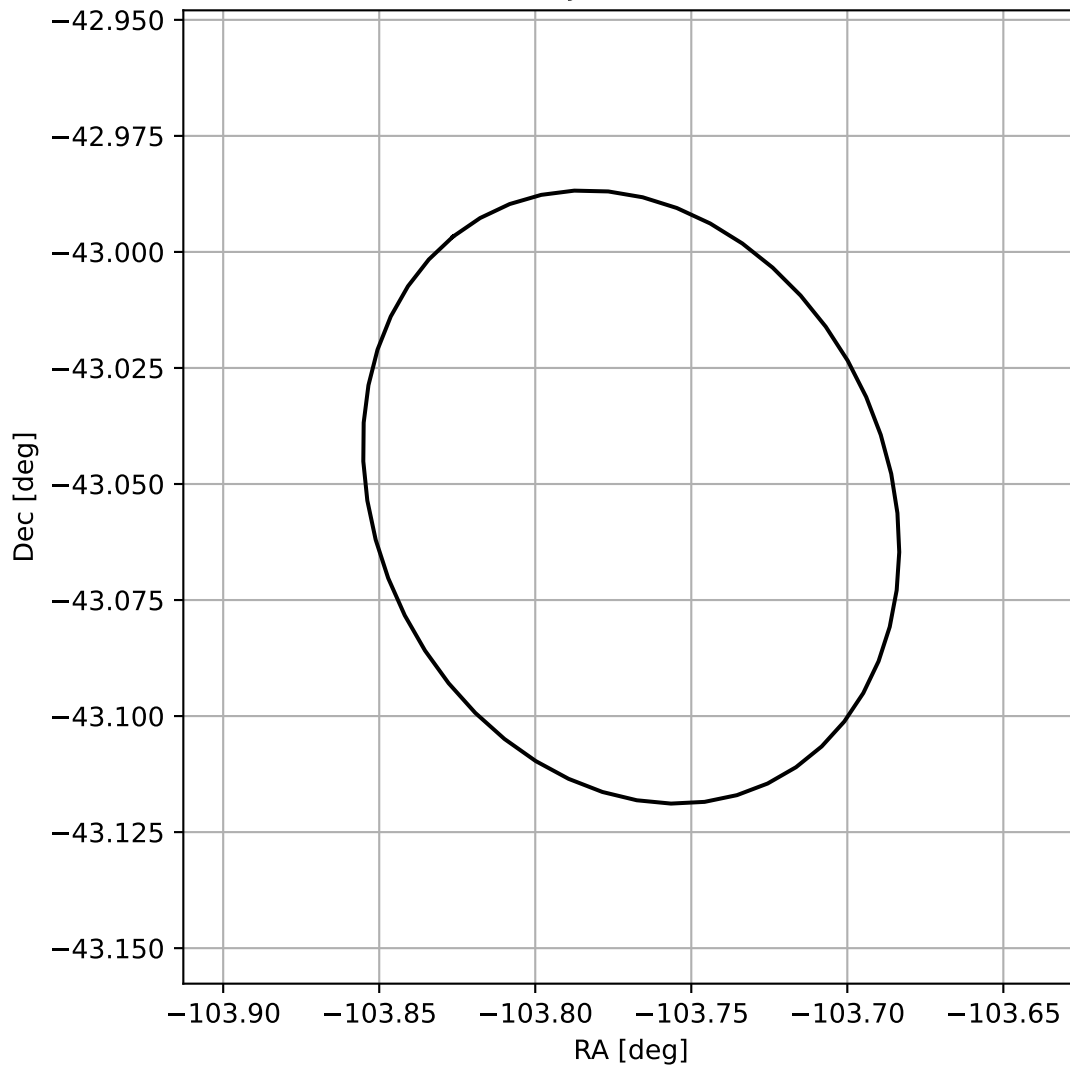
4FGL J1704.9-4303
