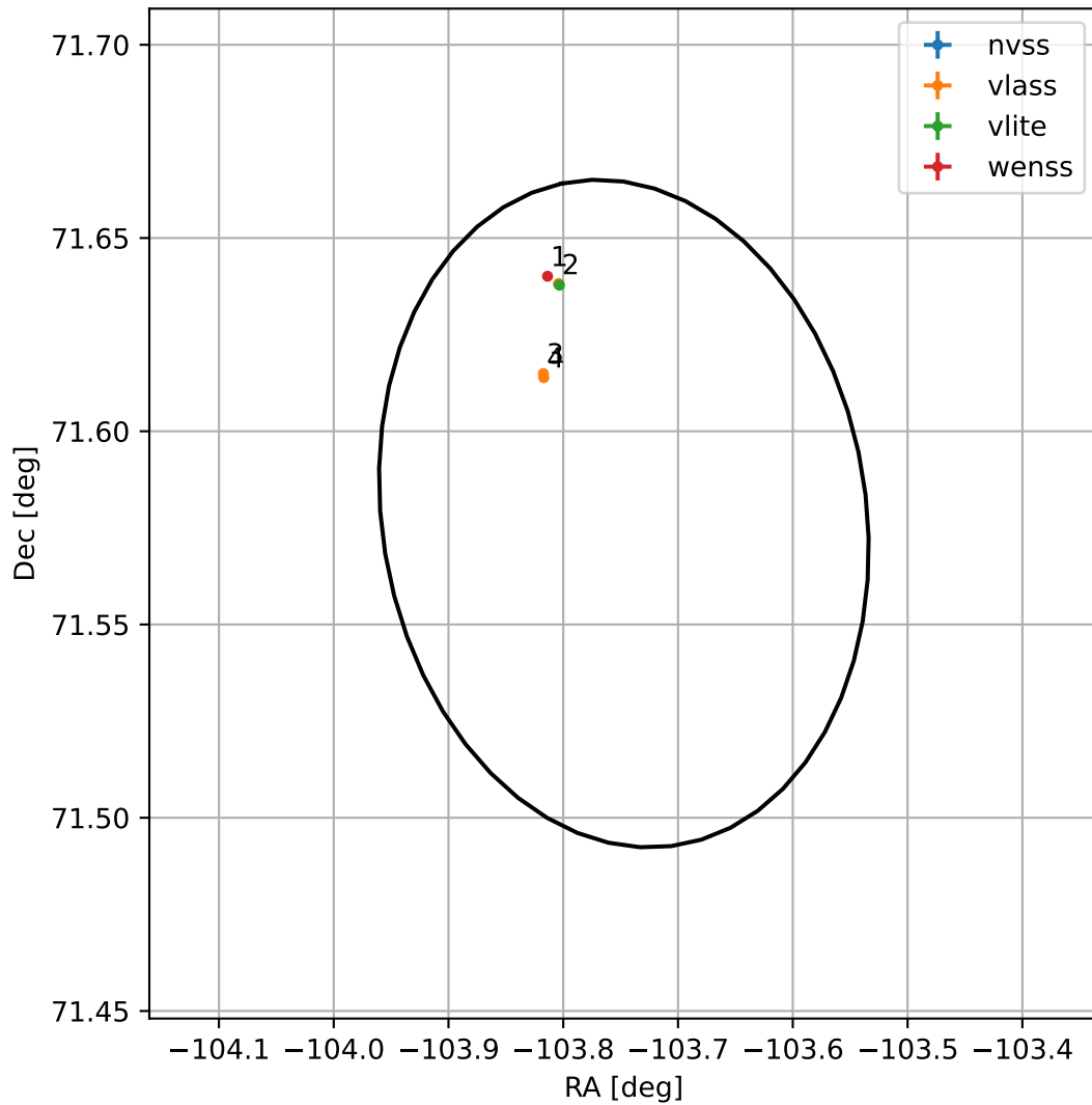
4FGL J1705.0+7134
