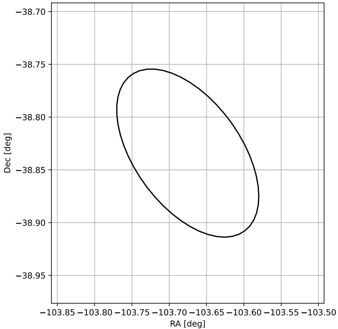
4FGL J1705.2-3850
