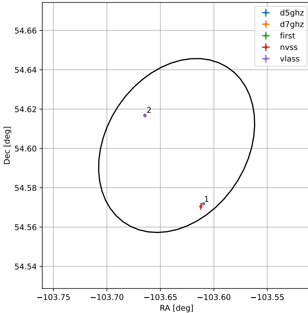
4FGL J1705.4+5436
