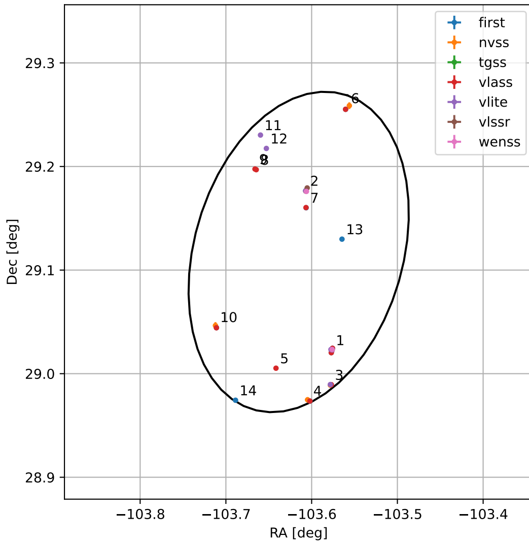
4FGL J1705.5+2907
