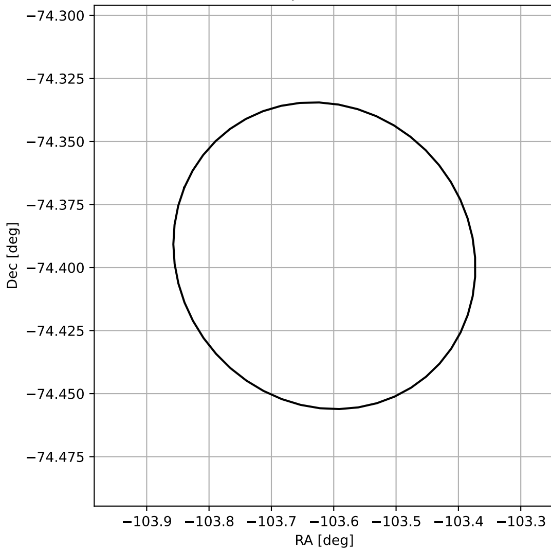
4FGL J1705.5-7423
