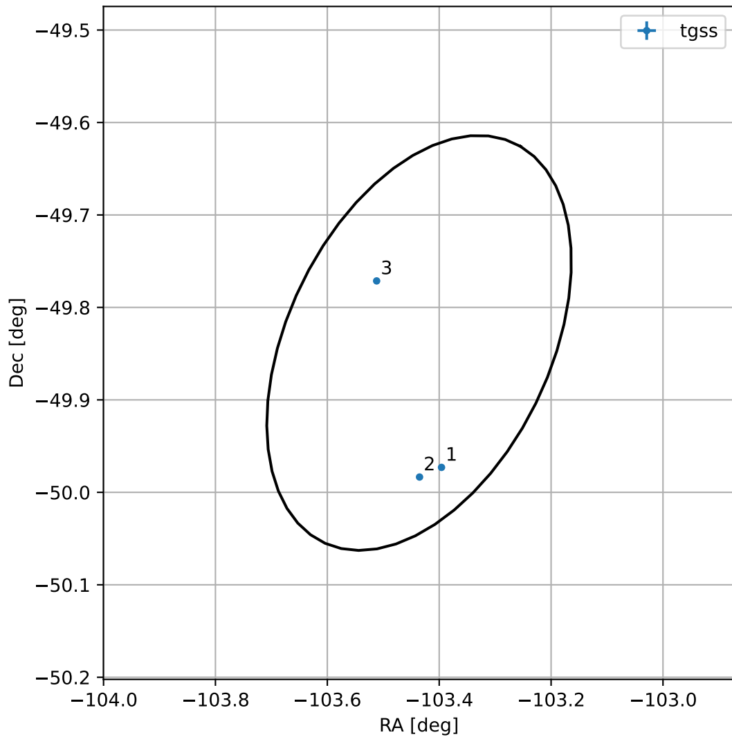
4FGL J1706.2-4950
