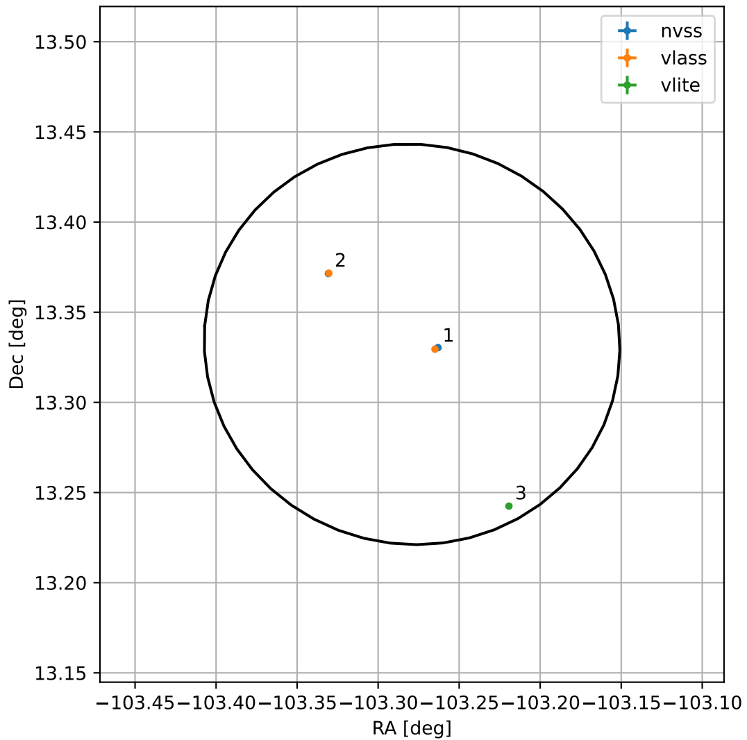
4FGL J1706.8+1319
