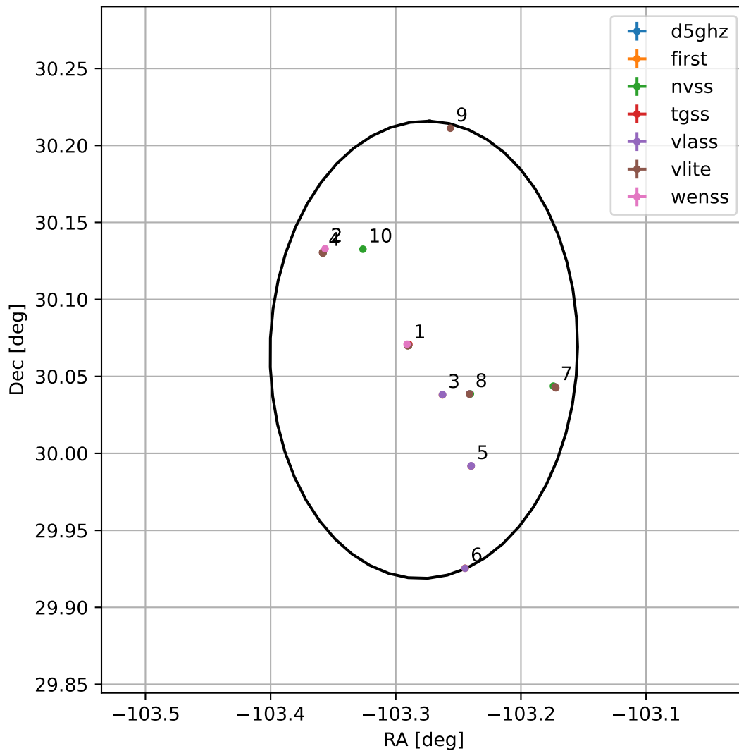
4FGL J1706.8+3004
