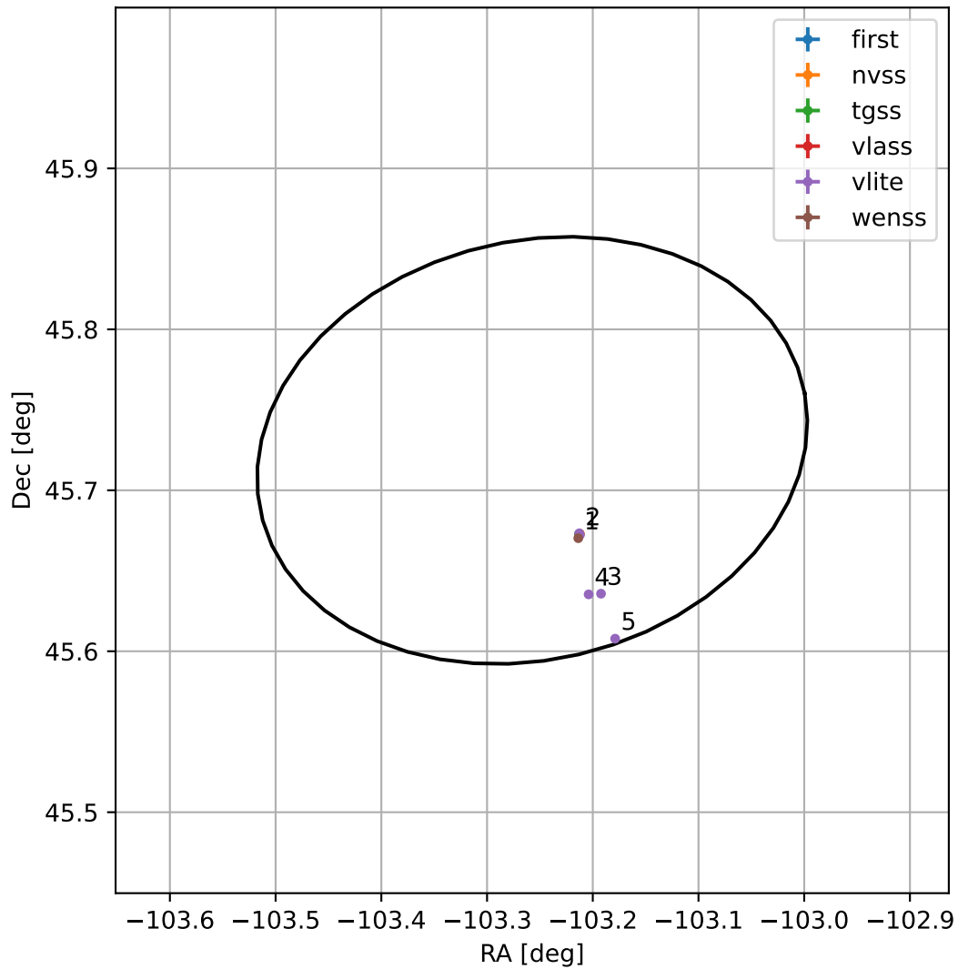
4FGL J1706.9+4543
