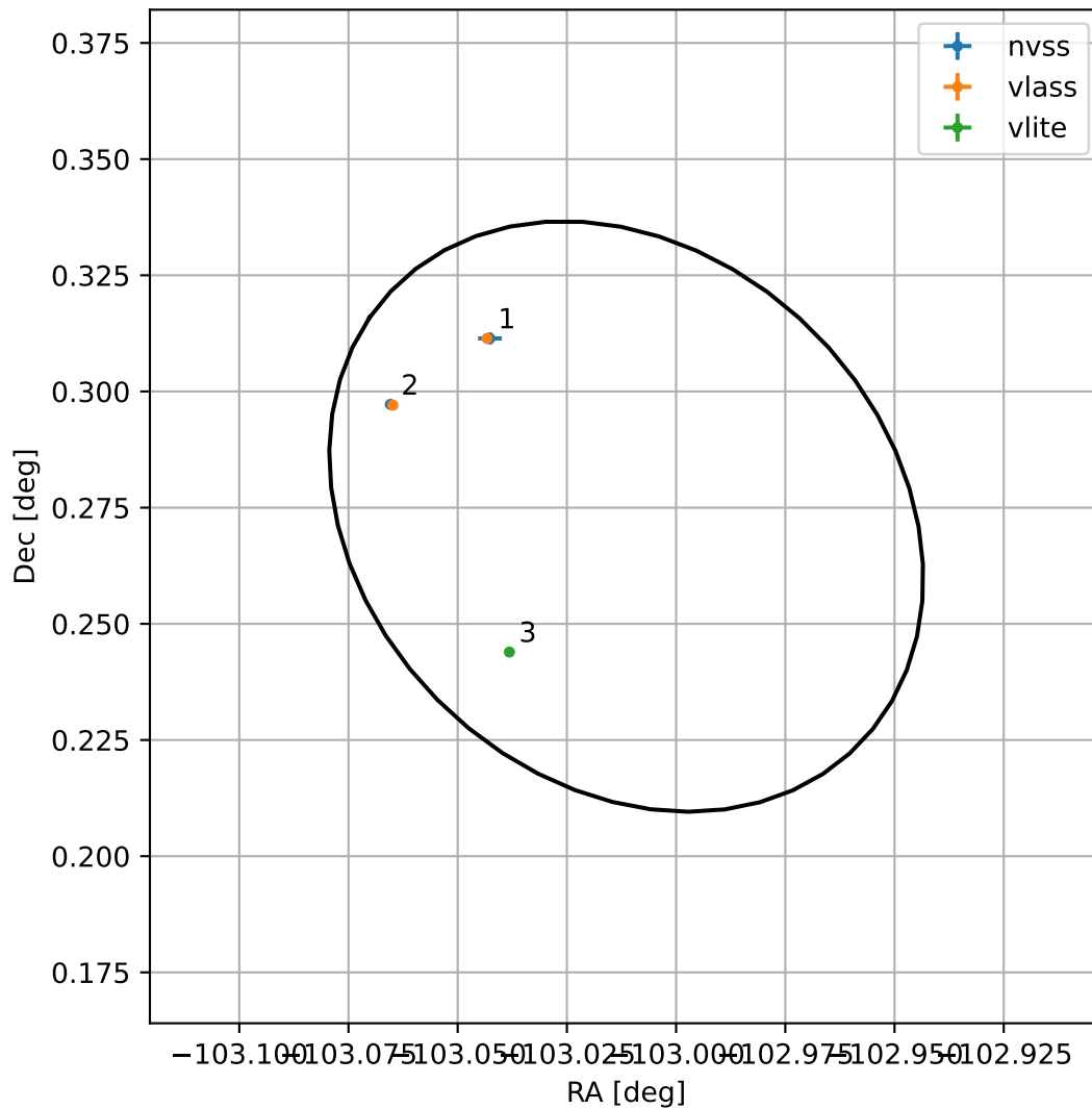
4FGL J1707.9+0016
