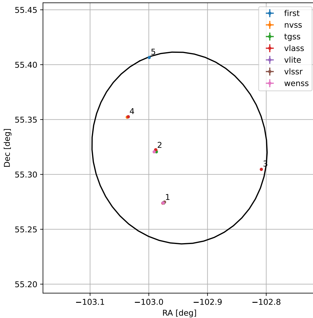
4FGL J1708.2+5519
