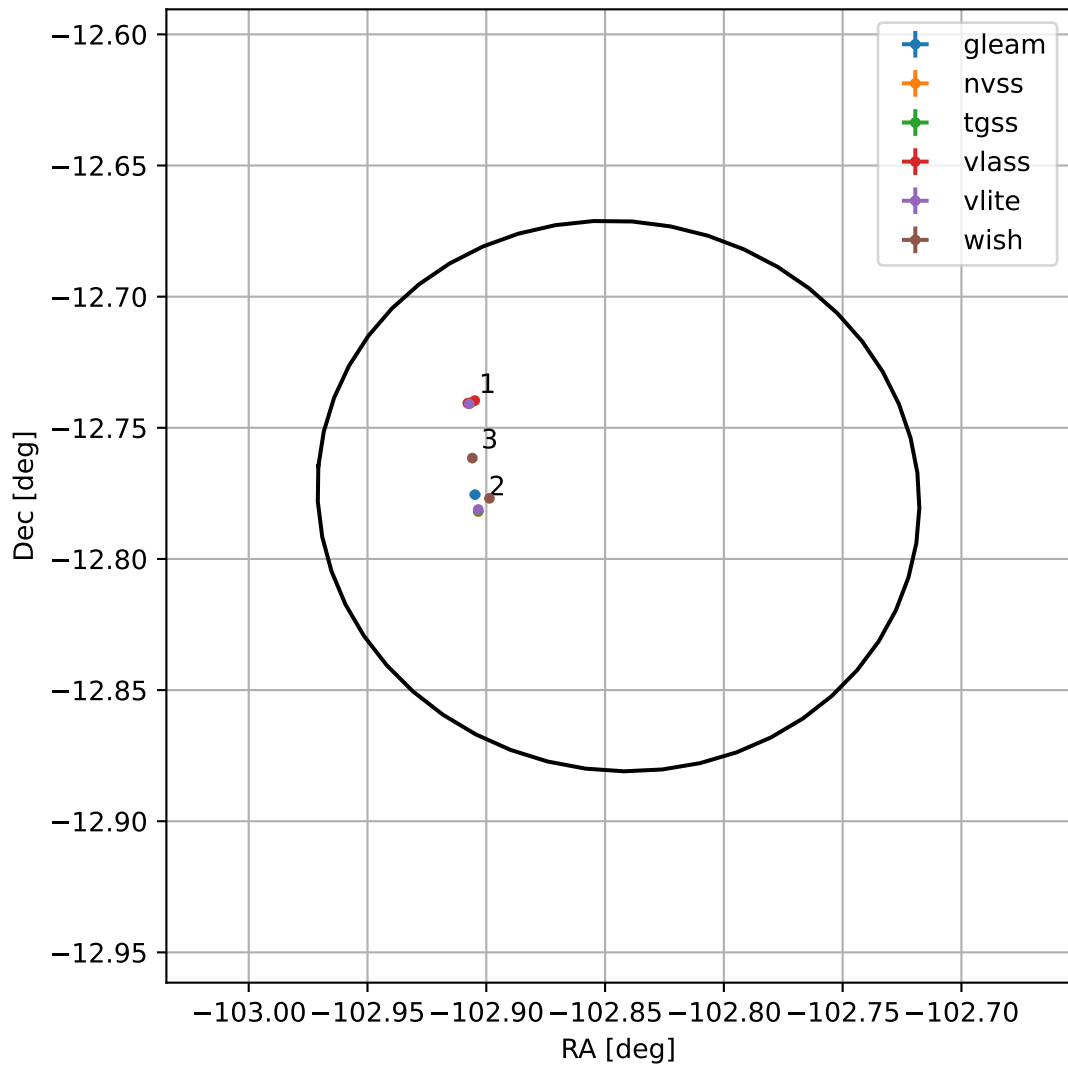
4FGL J1708.6-1246
