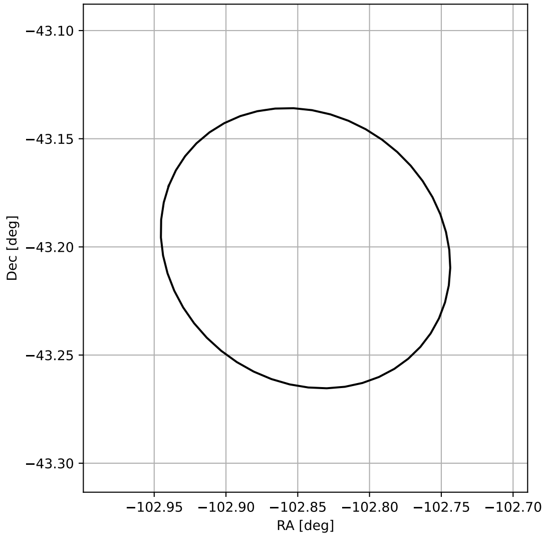
4FGL J1708.6-4312
