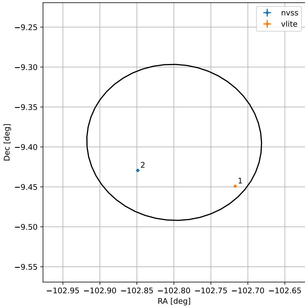
4FGL J1708.8-0923
