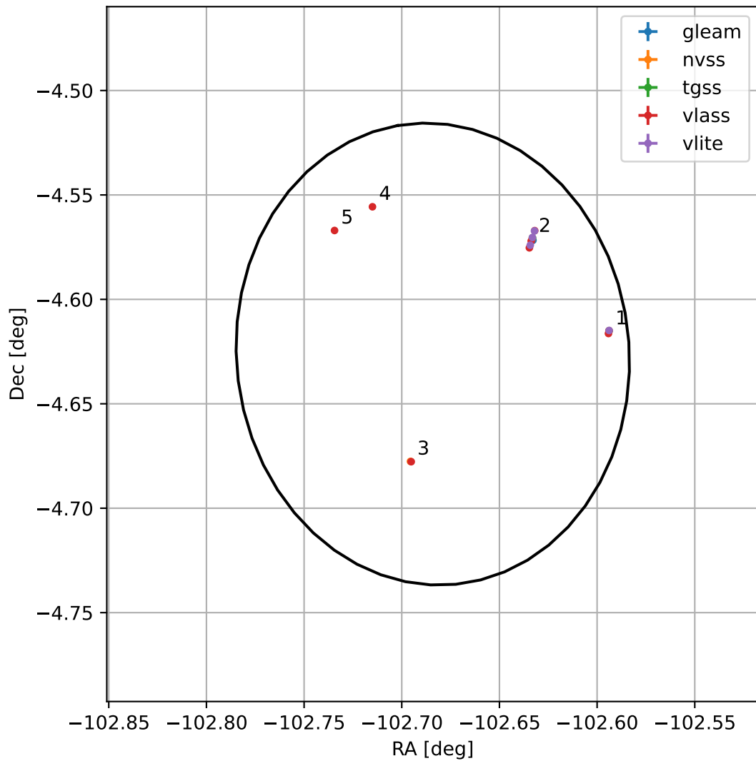
4FGL J1709.2-0437
