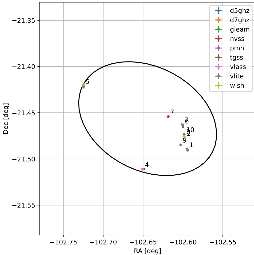
4FGL J1709.4-2127
