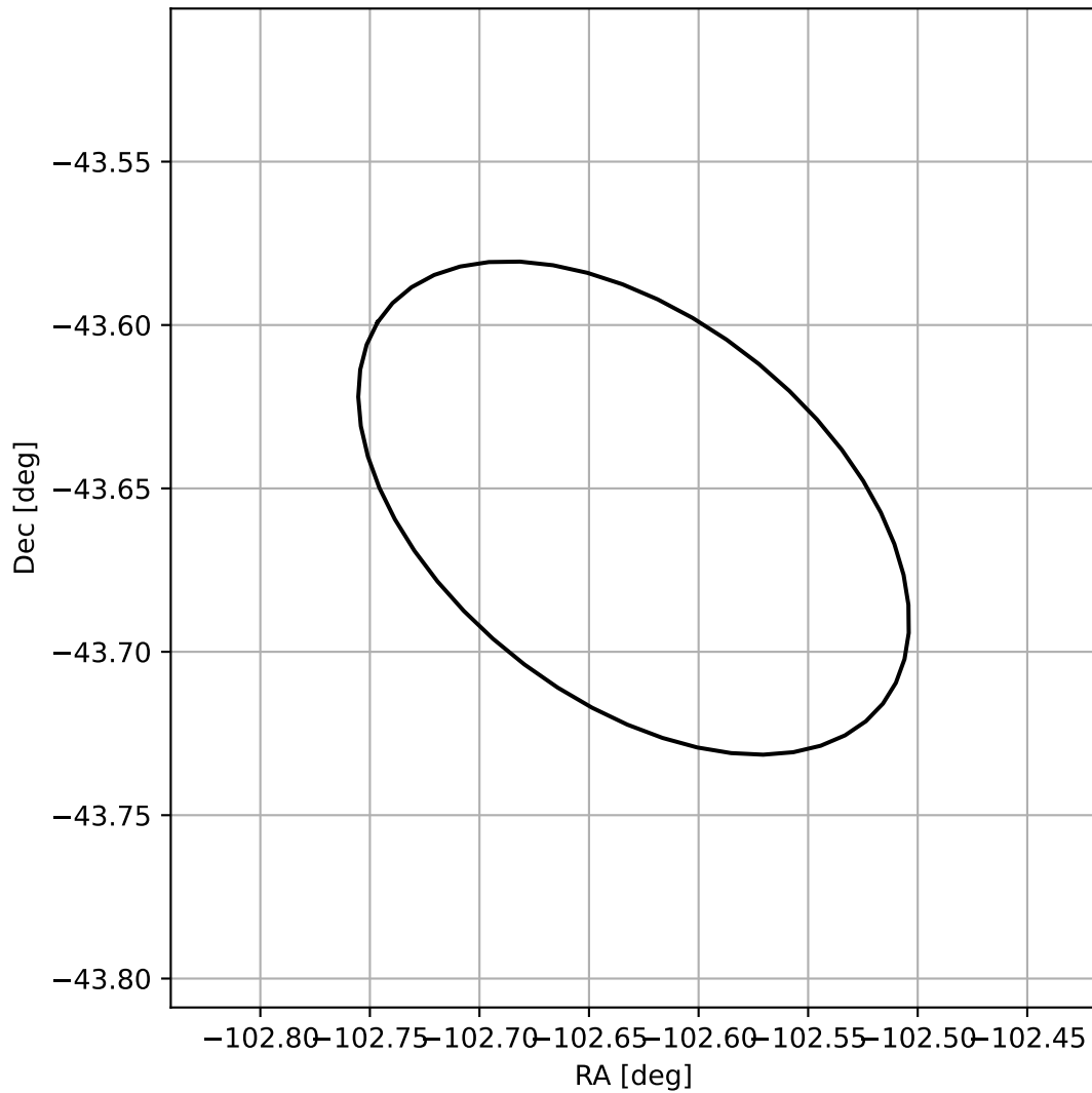
4FGL J1709.4-4339
