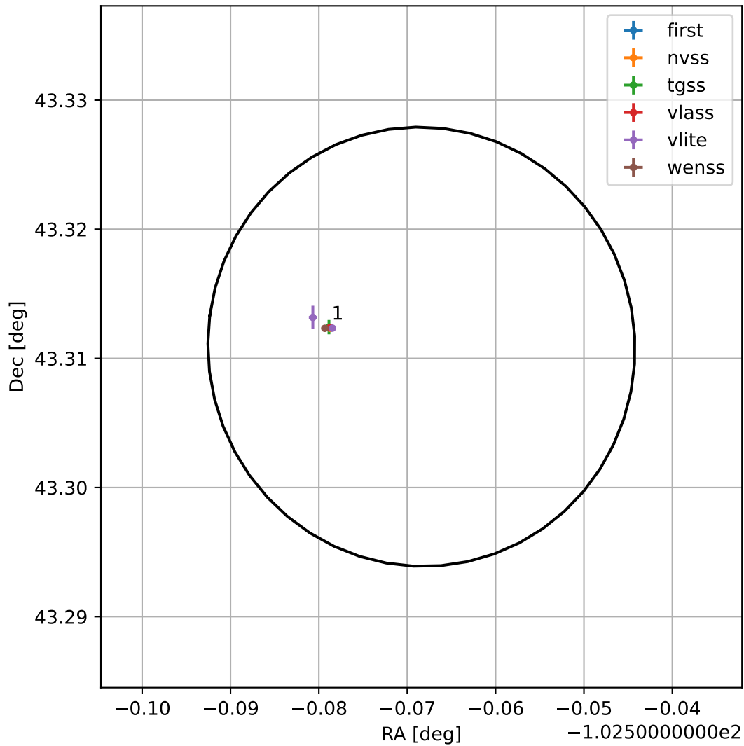
4FGL J1709.7+4318
