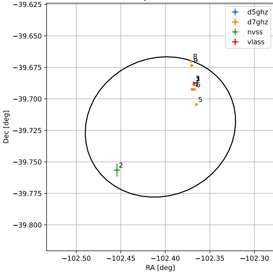
4FGL J1710.3-3943
