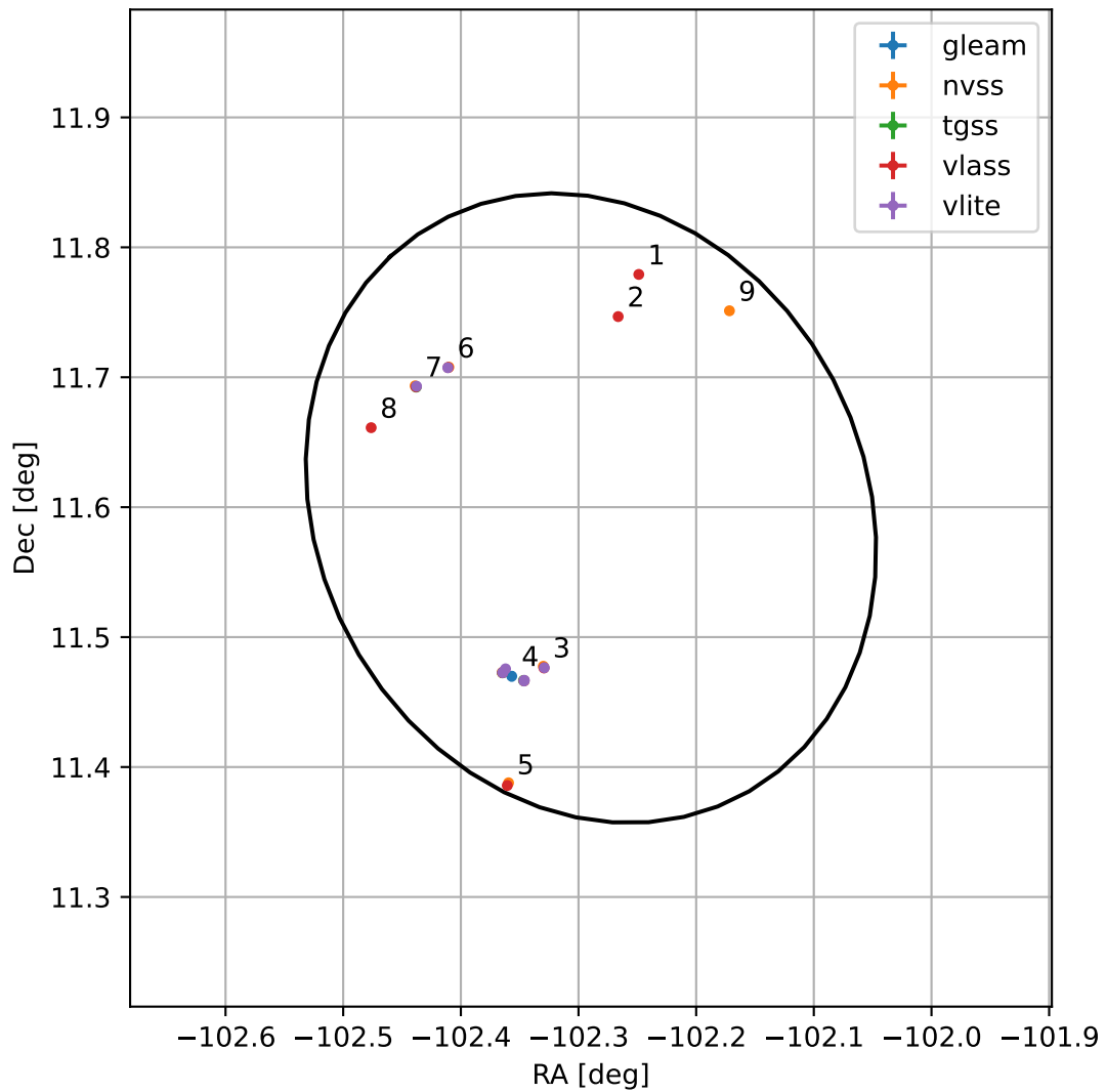
4FGL J1710.8+1135
