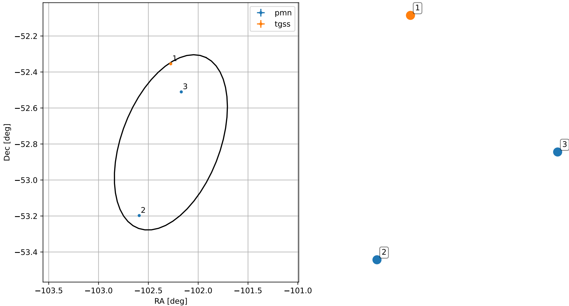
4FGL J1710.9-5247
